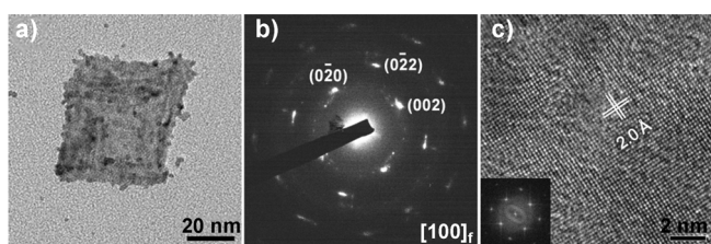
Figure 3. a) Bright-field TEM image and b) the corresponding SAED pattern of a typical fcc Au@Pt square nanoplate with (100)_f orientation. c) Typical HRTEM image of a fcc Au@Pt square nanoplate. Scale bar = 2 nm. Inset in (c): the corresponding FFT pattern for the HRTEM image shown in (c).
